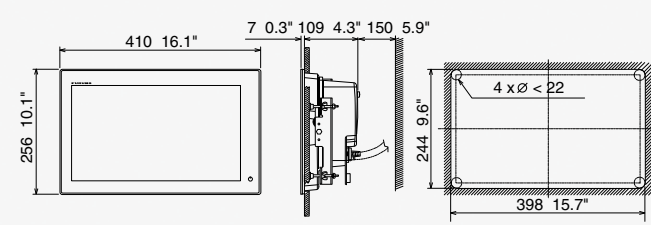
Multi Function Display (Flush Mount) TZTL15F 4.9 kg 10.8 lb
